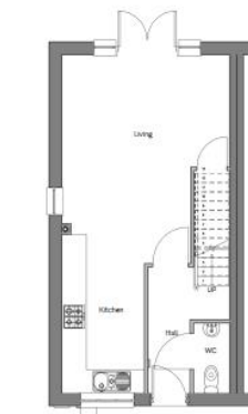
Ground Floor - Planning
