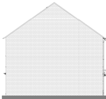
Left Elevation. 1:50
